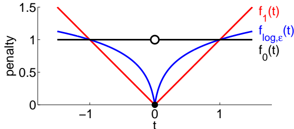
Figure 3: At the origin, the canonical \ell_0 sparsity count f_0(t) is better approximated by the log-sum penalty function f_{\log,\epsilon}(t) than by the traditional convex \ell_1 relaxation f_1(t) .
