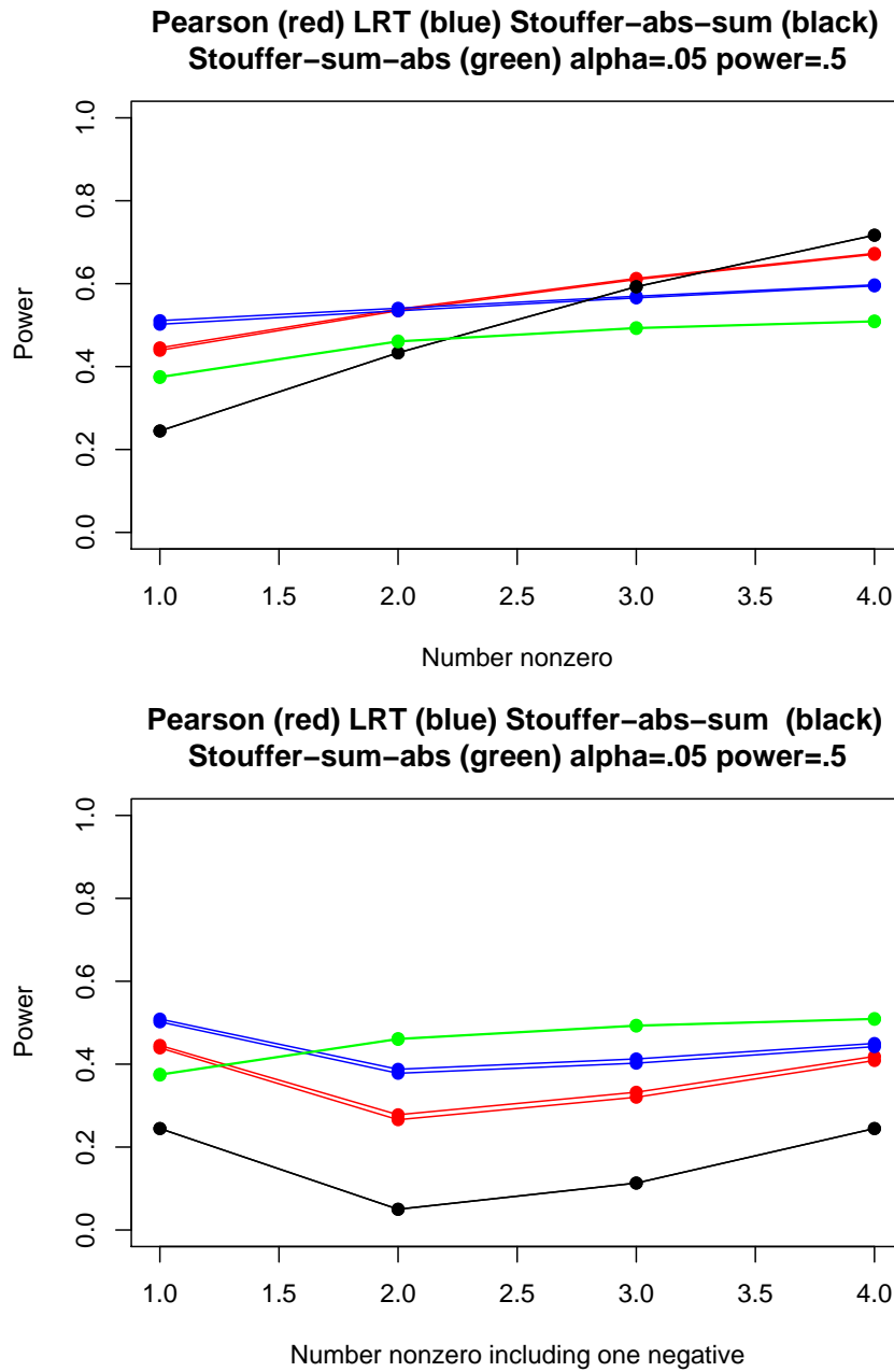
FIG 16. The top figure shows power curves for m = 4 with \alpha = 0.05 and \Delta chosen so that a chisquare test has power 0.5. The alternative is concordant. The bottom figure shows the nearly concordant alternative.
